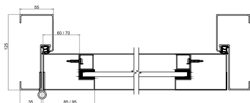
Single Door Section
