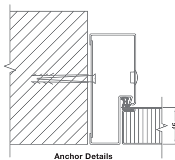
Anchor Details
